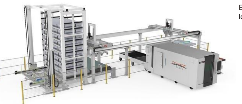
Enclosed type fiber laser cutting machine with automatic loading and unloading material warehouse
